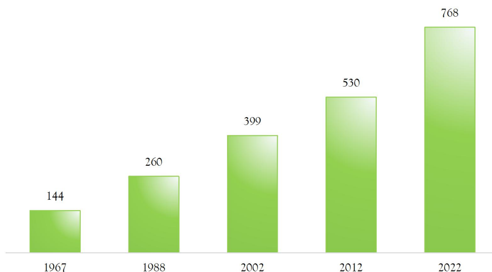
Figure C.1.4: Population Density, 1967- 2022
